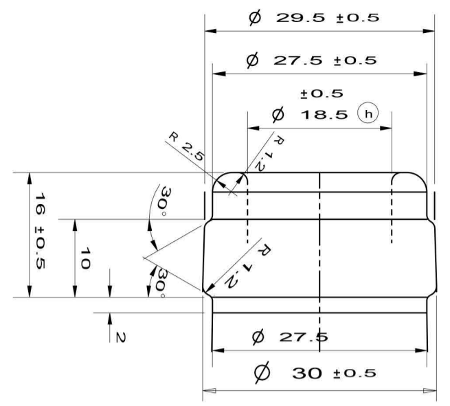
NECK DETAILS
