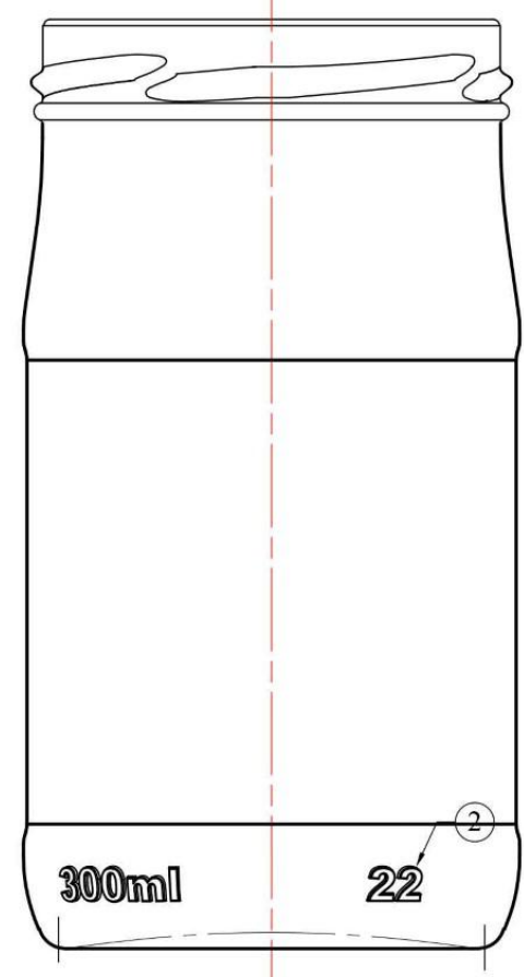
VIEW C SCALE 1 : 1
